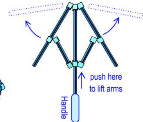
Working model of umbrella mechanism. An example of an animated shape
